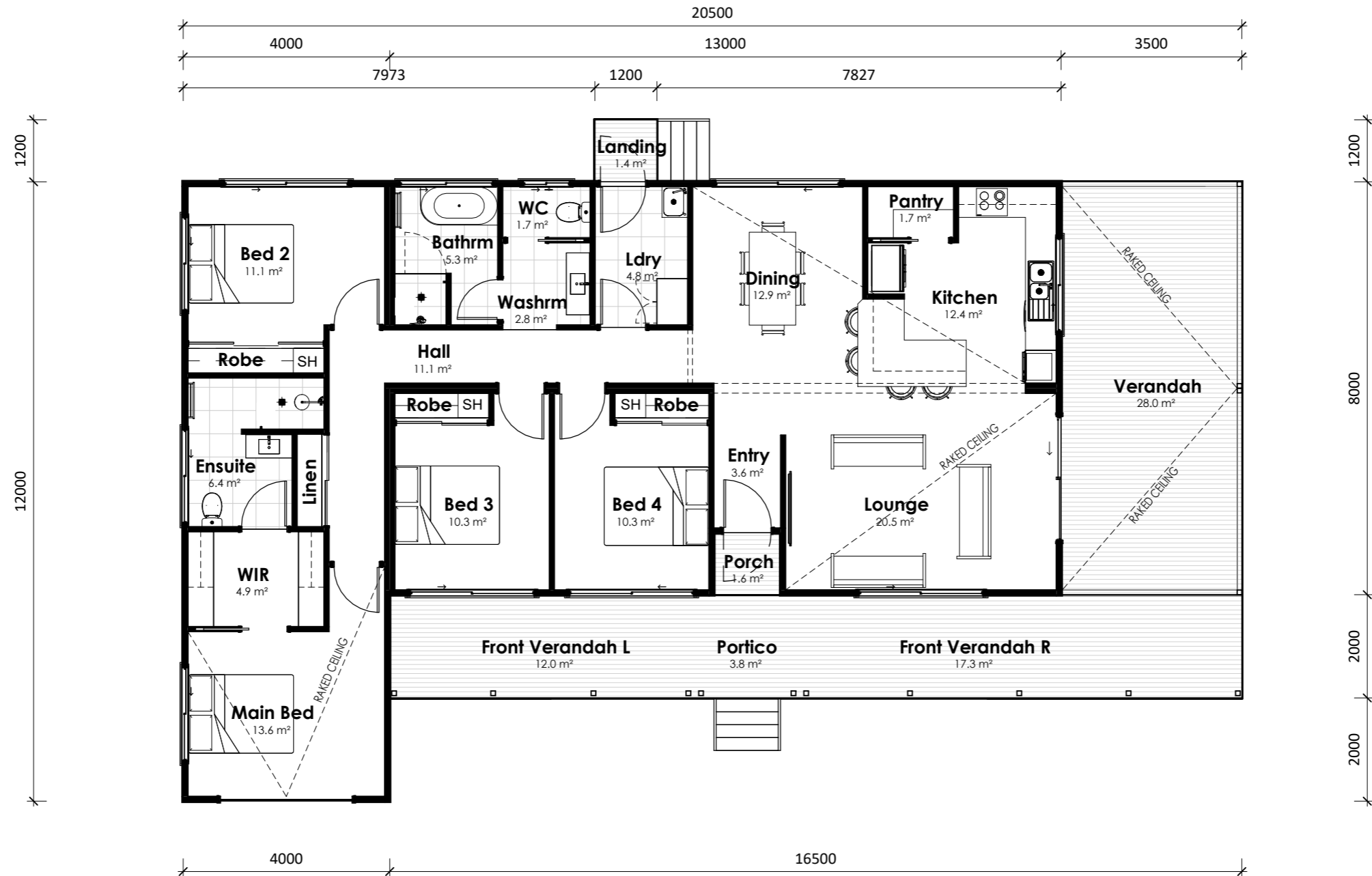
FLOOR PLAN 1:100
