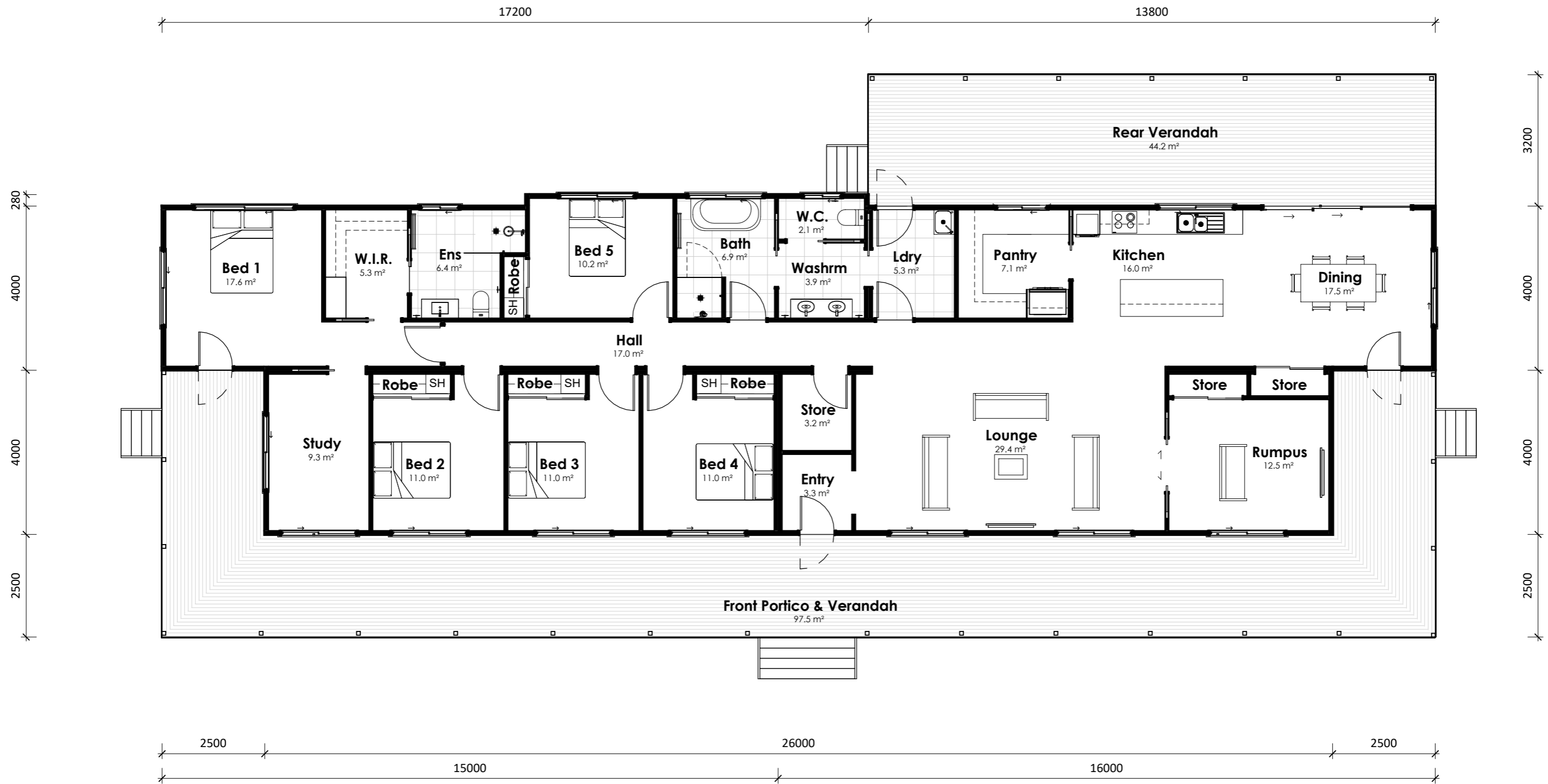
FLOOR PLAN 1:100
